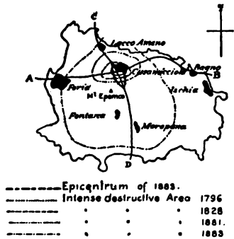
FIG. 81. — Map of the island of Ischia to show how the shocks of recent earthquakes have been concentrated at the crossing point of two fractures (after Mercalli and Johnston-Lavis).
